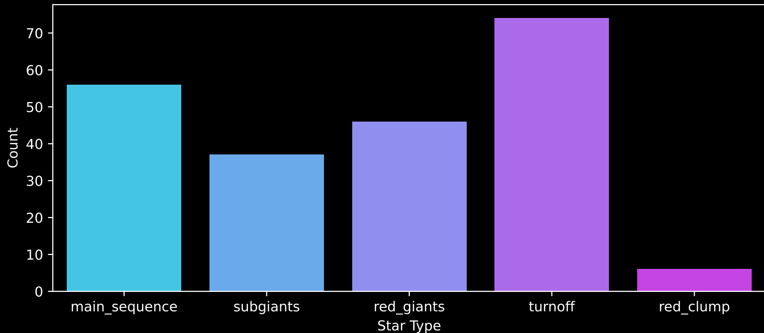
GALAH DR4 Field: [8488] Count plot of Star Type
