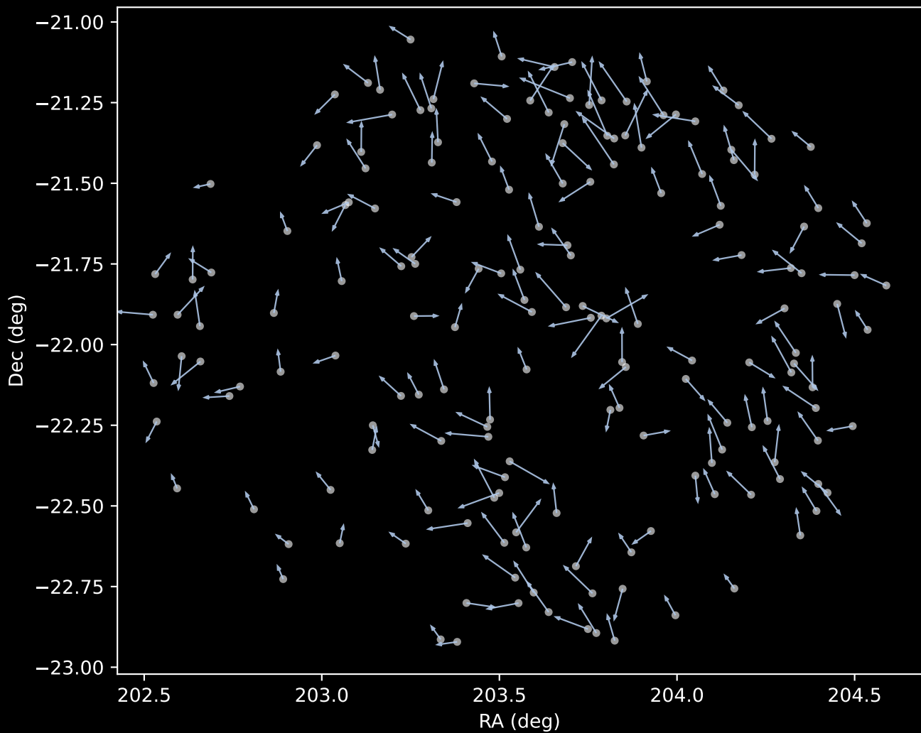
GALAH DR4 Cluster 1 Proper Motion Vectors (n=176)
