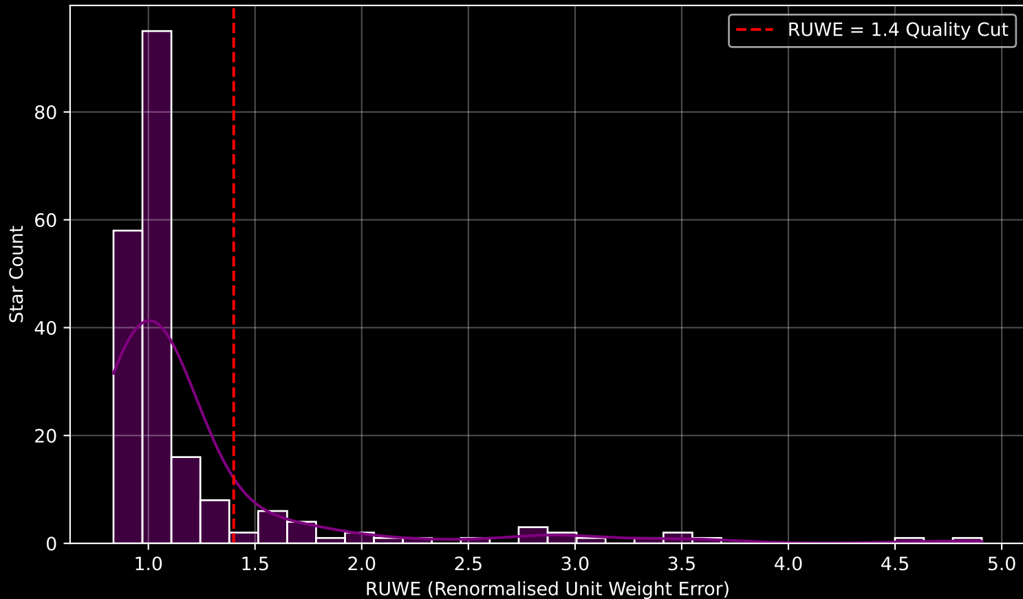
GALAH DR4 Field [8488] RUWE Distribution (n= 207)
