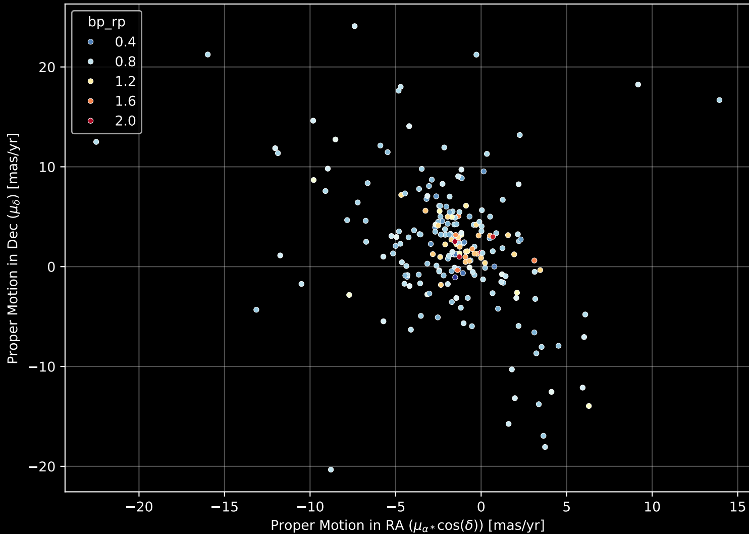
GALAH DR4 Field: [8488] Proper Motion Diagram (n= 219)
